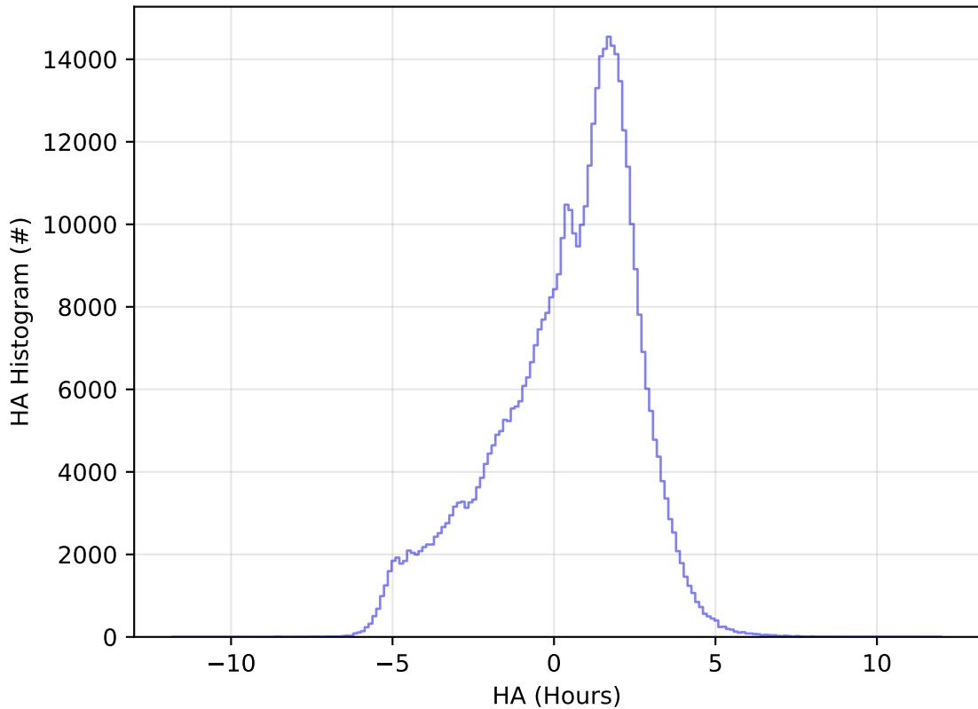
early_u_fpextra2.0_v3.4_10yrs All sky r band: HA Histogram
