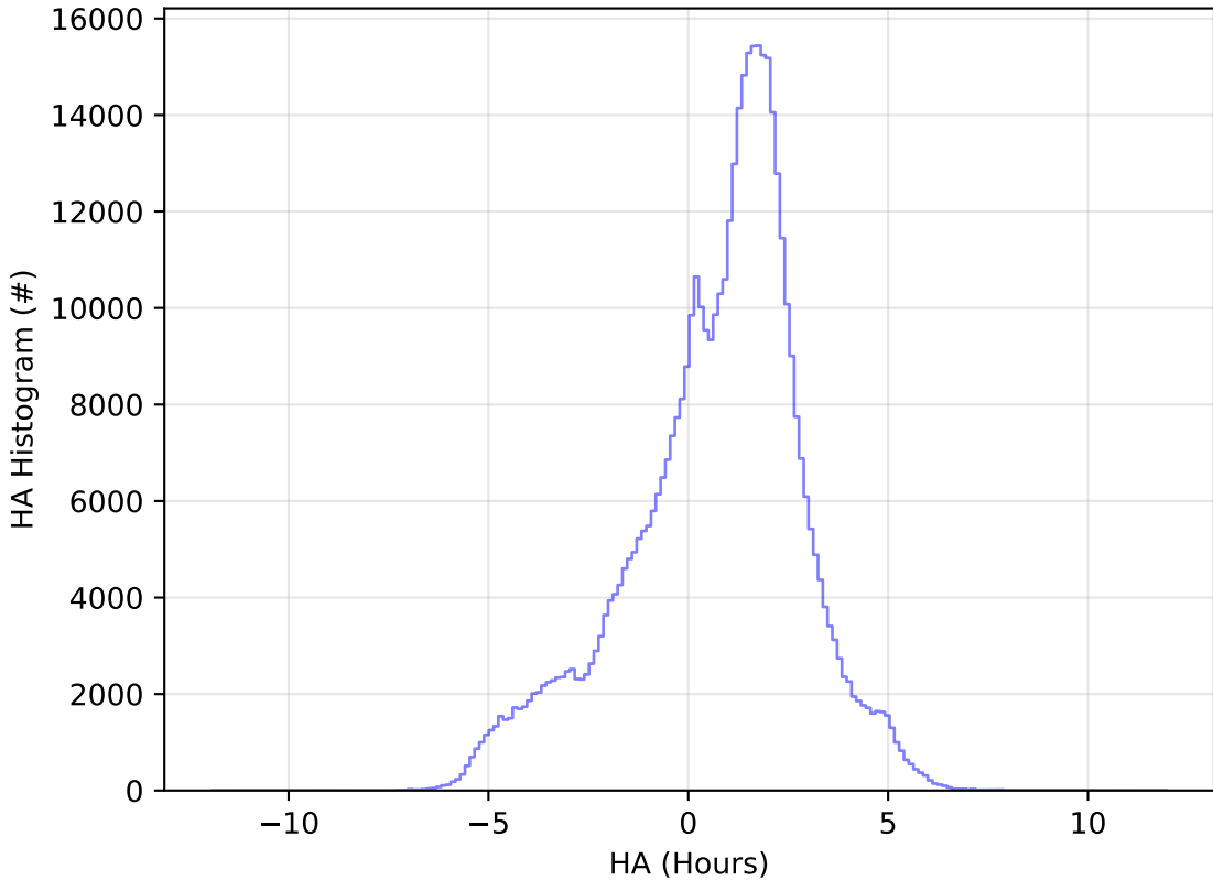
early_u_fpextra2.0_v3.4_10yrs All sky i band: HA Histogram
