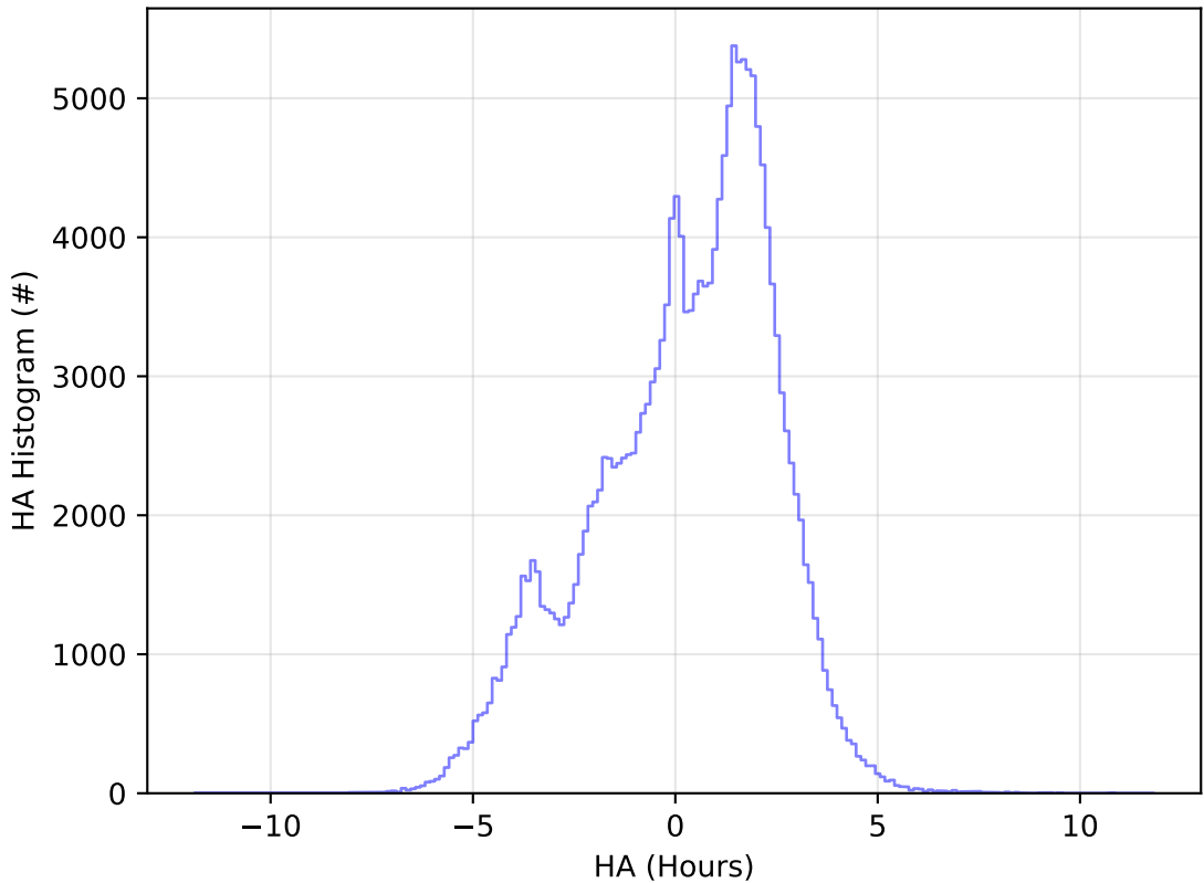
early_u_fpextra2.0_v3.4_10yrs All sky g band: HA Histogram
