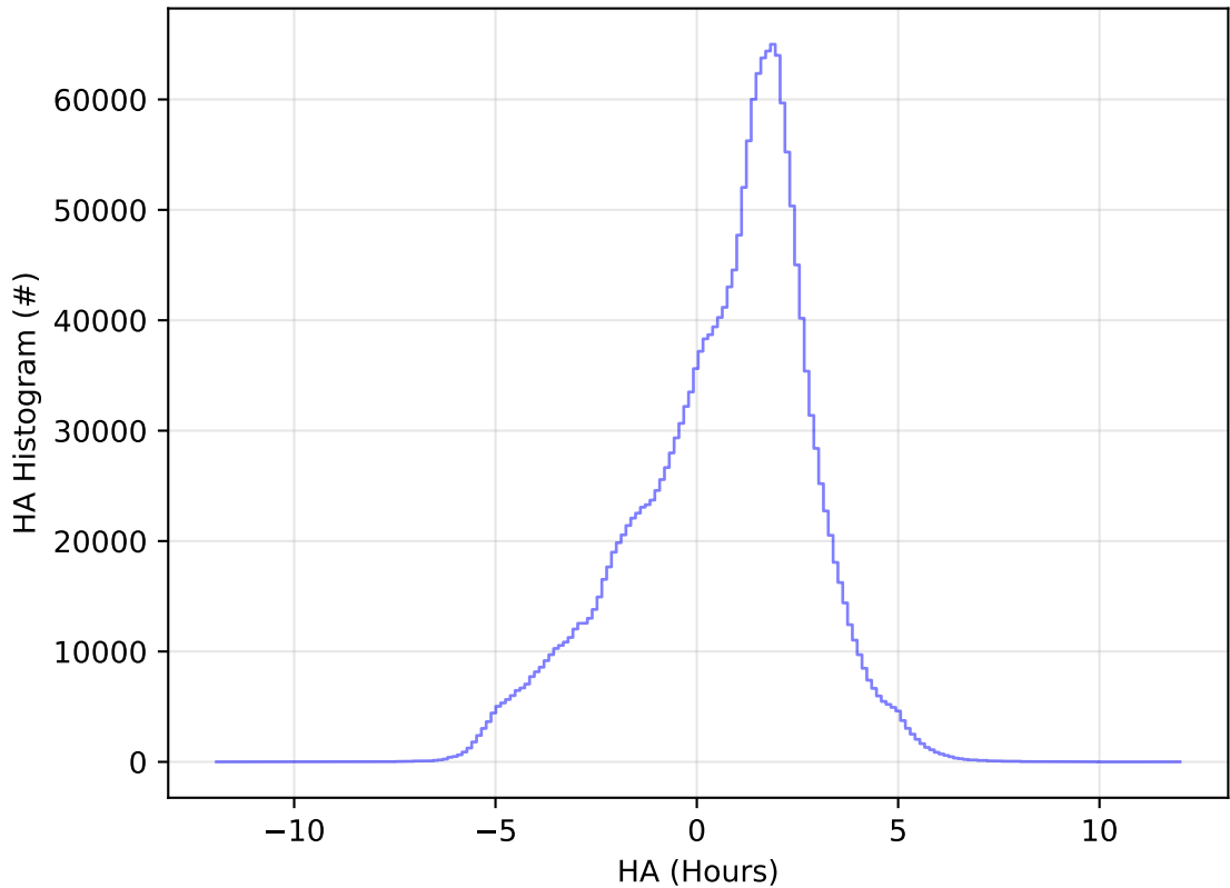
early_u_fpextra2.0_v3.4_10yrs All sky all bands: HA Histogram
