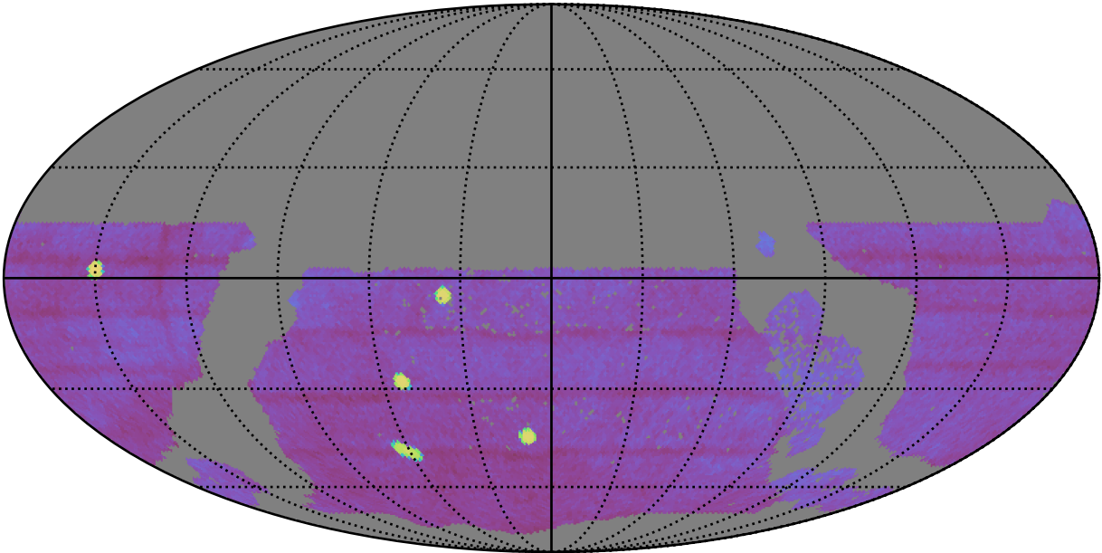
early_u_fpextra2.0_v3.4_10yrs gri WFD: Fraction of visits with a revisit < 60 min
