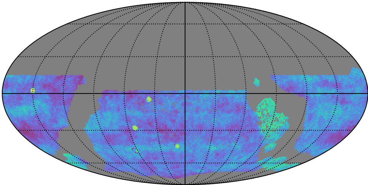
early_u_fpextra2.0_v3.4_10yrs gri WFD: Fraction of visits in pairs (20-90 min)
