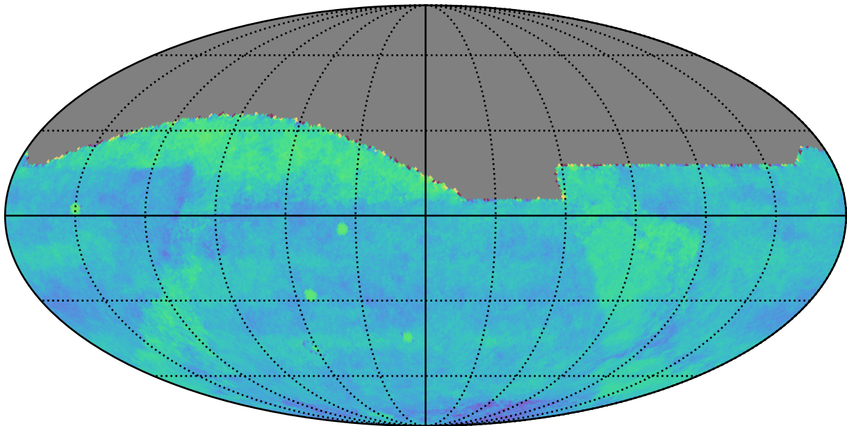
early_u_fpextra2.0_v3.4_10yrs gri All sky: Fraction of visits in pairs (20-90 min)
