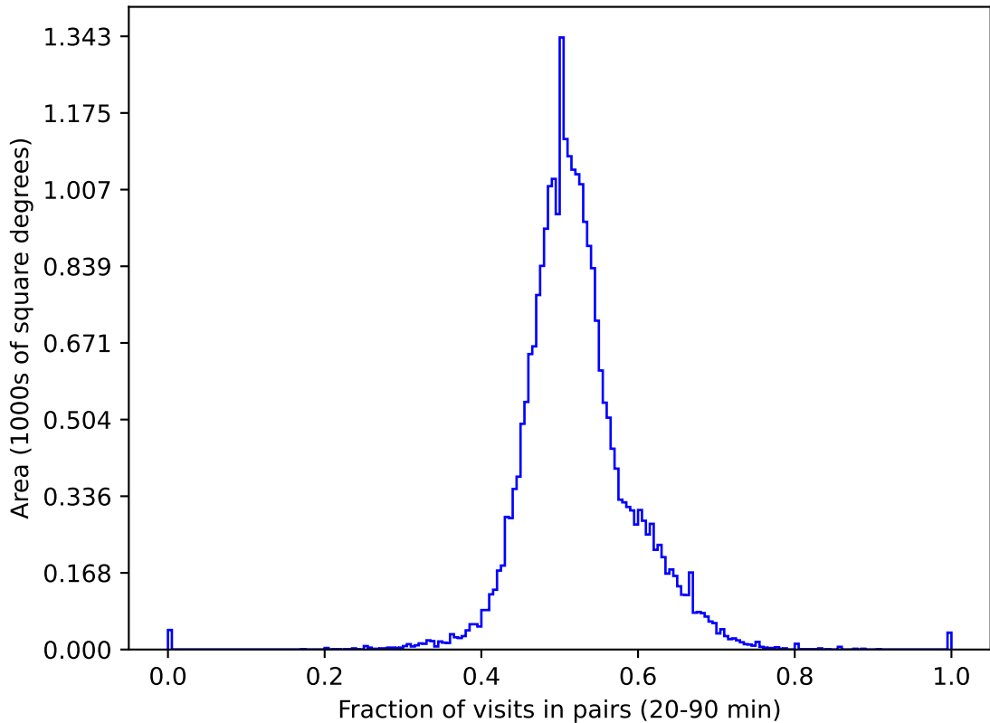
early_u_fpextra2.0_v3.4_10yrs gri All sky: Fraction of visits in pairs (20-90 min)
