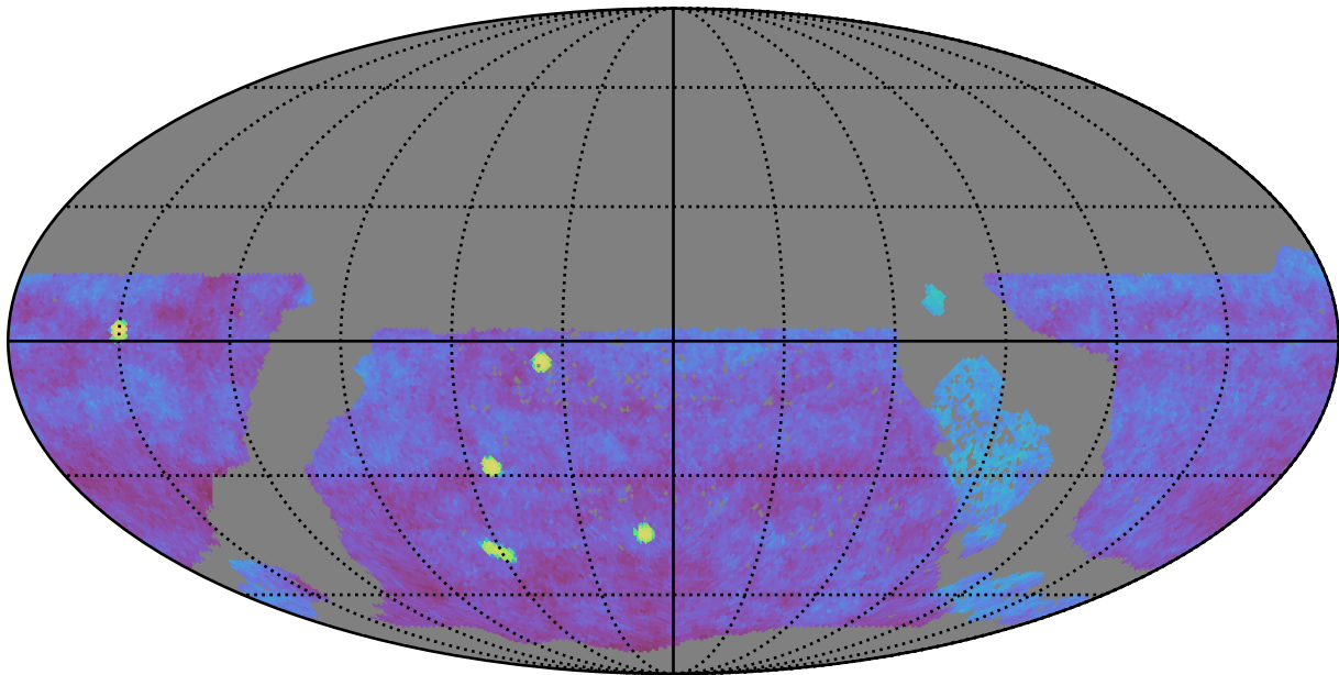
early_u_fpextra2.0_v3.4_10yrs gri WFD: Fraction of visits in pairs (10-60 min)
