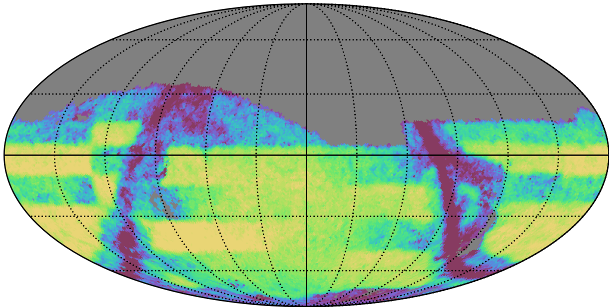
early_u_fpextra2.0_v3.4_10yrs Yr 3-4 z band: Exgal_CoaddM5
