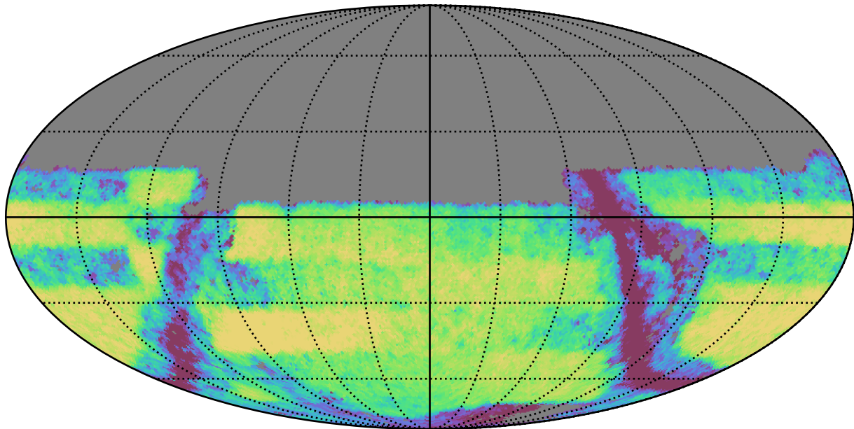
early_u_fpextra2.0_v3.4_10yrs Yr 3-4 y band: Exgal_CoaddM5
