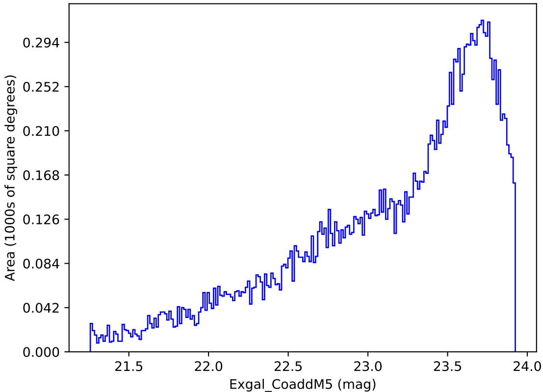
early_u_fpextra2.0_v3.4_10yrs Yr 3-4 y band: Exgal_CoaddM5
