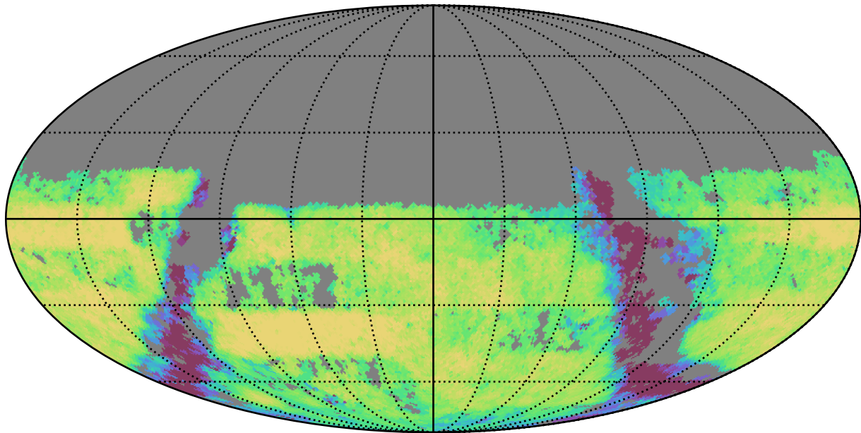
early_u_fpextra2.0_v3.4_10yrs Yr 3-4 u band: Exgal_CoaddM5
