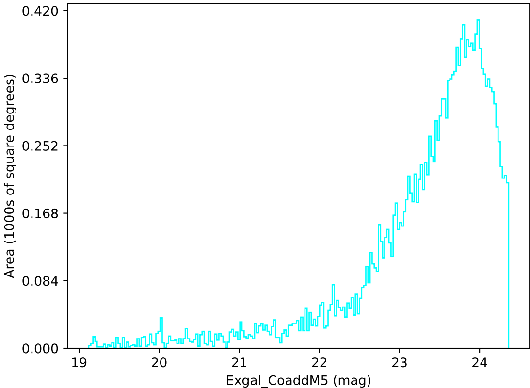
early_u_fpextra2.0_v3.4_10yrs Yr 3-4 u band: Exgal_CoaddM5
