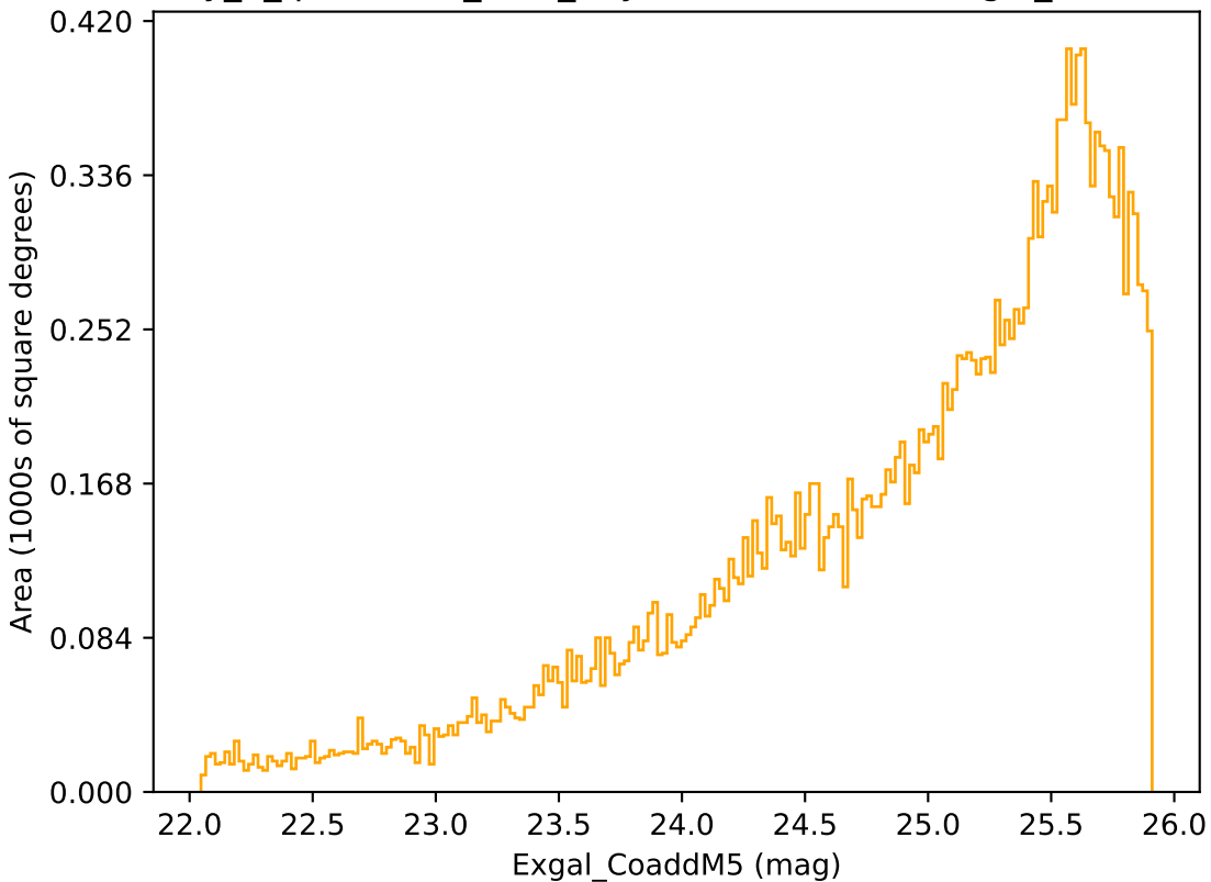
early_u_fpextra2.0_v3.4_10yrs Yr 3-4 r band: Exgal_CoaddM5
