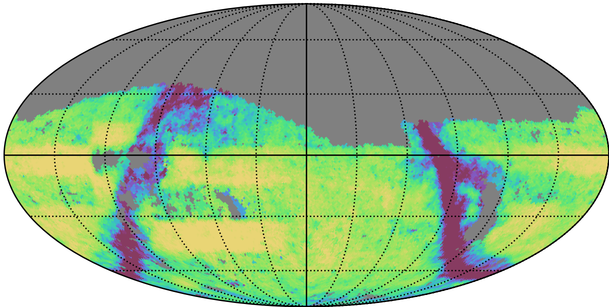
early_u_fpextra2.0_v3.4_10yrs Yr 3-4 g band: Exgal_CoaddM5
