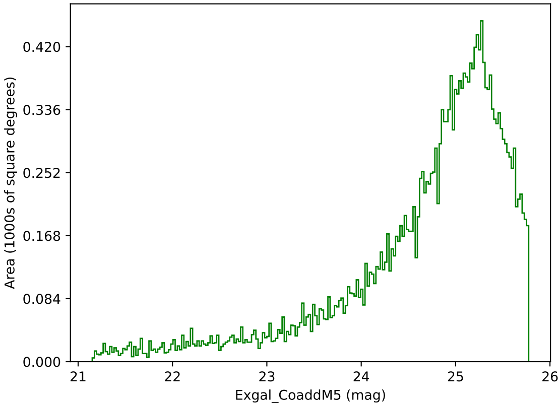
early_u_fpextra2.0_v3.4_10yrs Yr 3-4 g band: Exgal_CoaddM5
