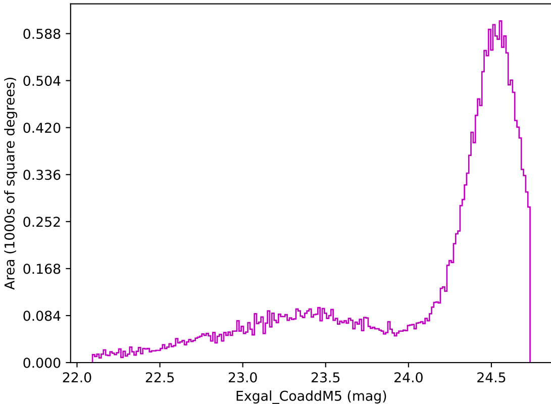
early_u_fpextra2.0_v3.4_10yrs Yr 1 z band: Exgal_CoaddM5
