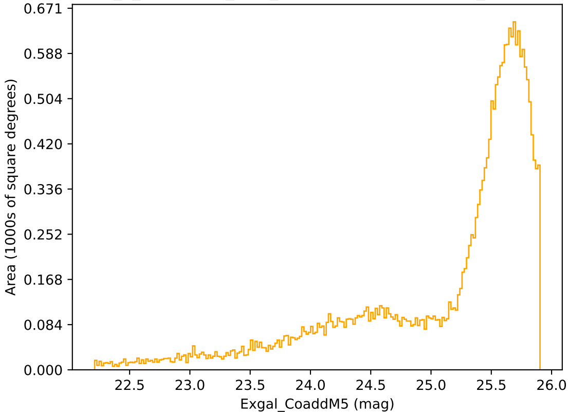
early_u_fpextra2.0_v3.4_10yrs Yr 1 r band: Exgal_CoaddM5
