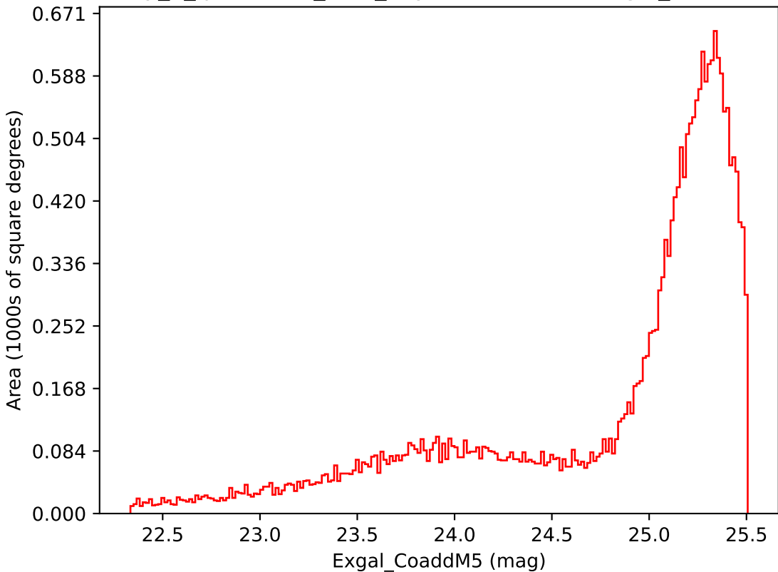
early_u_fpextra2.0_v3.4_10yrs Yr 1 i band: Exgal_CoaddM5
