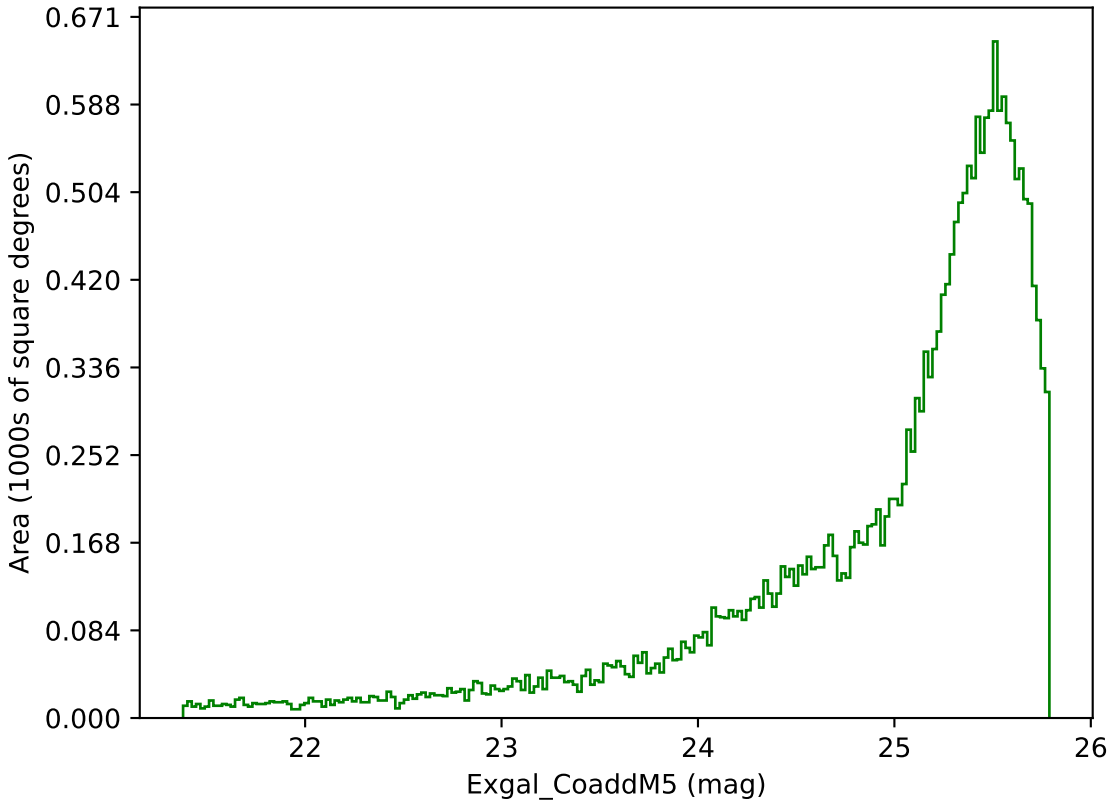
early_u_fpextra2.0_v3.4_10yrs Yr 1 g band: Exgal_CoaddM5
