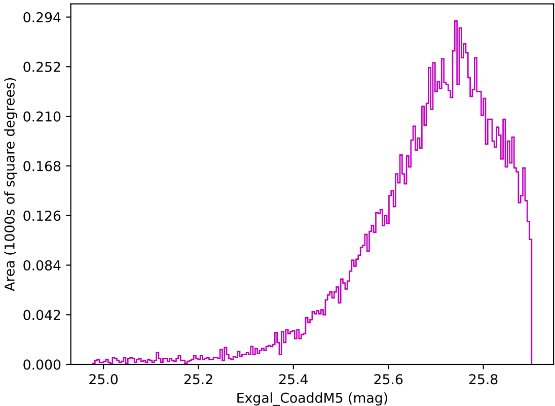
early_u_fpextra2.0_v3.4_10yrs WFD z band: Exgal_CoaddM5
