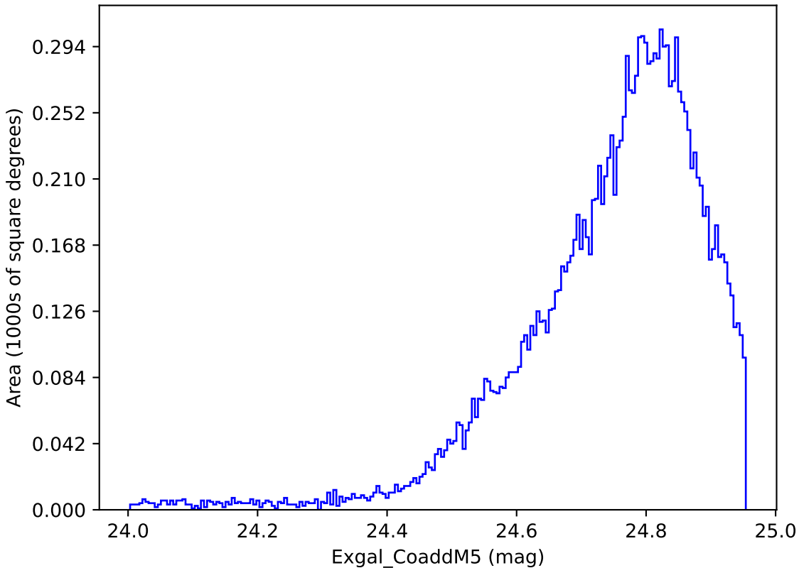
early_u_fpextra2.0_v3.4_10yrs WFD y band: Exgal_CoaddM5
