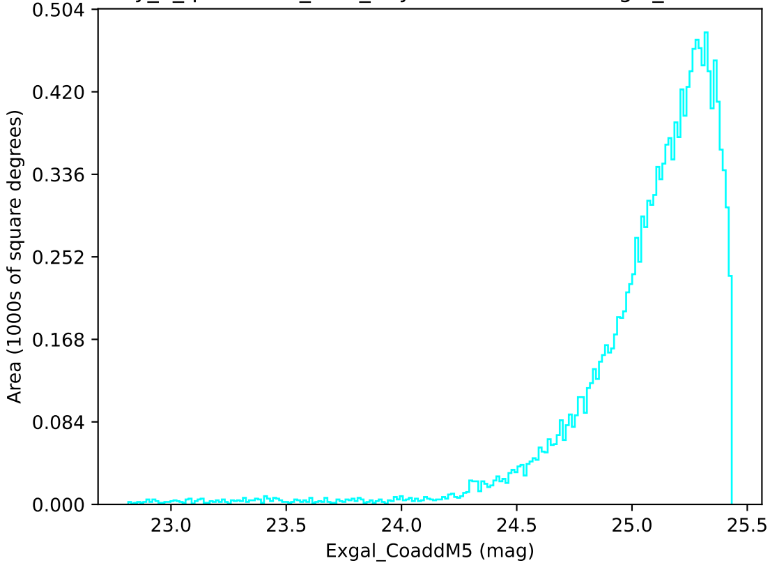
early_u_fpextra2.0_v3.4_10yrs WFD u band: Exgal_CoaddM5
