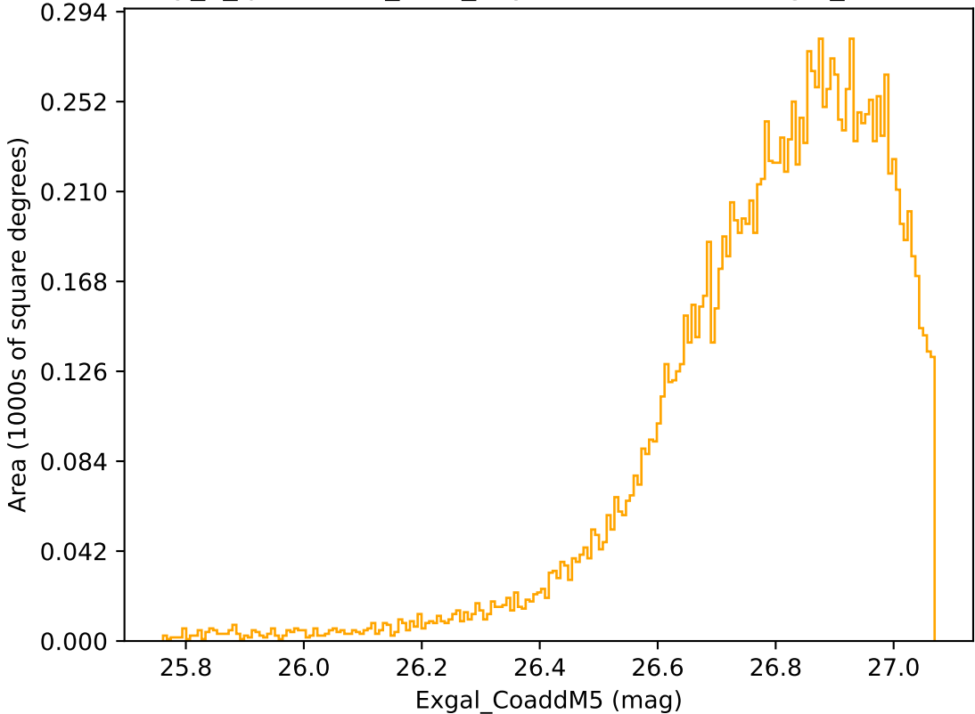
early_u_fpextra2.0_v3.4_10yrs WFD r band: Exgal_CoaddM5
