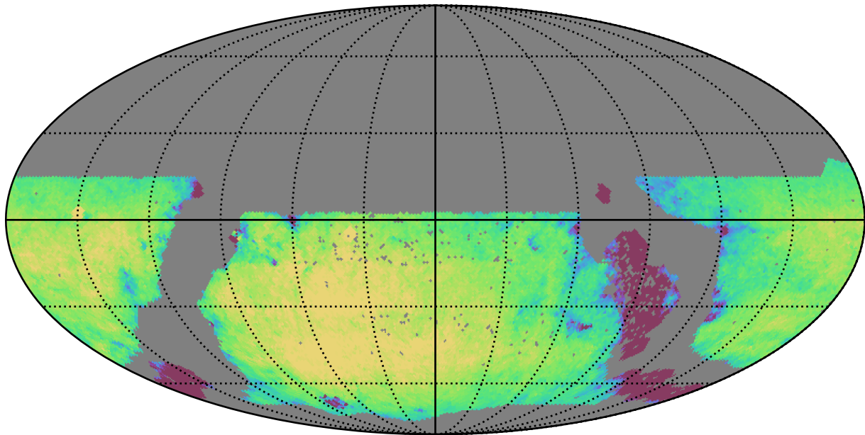
early_u_fpextra2.0_v3.4_10yrs WFD g band: Exgal_CoaddM5
