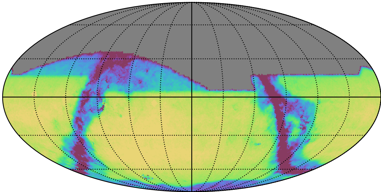
early_u_fpextra2.0_v3.4_10yrs All sky z band: Exgal_CoaddM5
