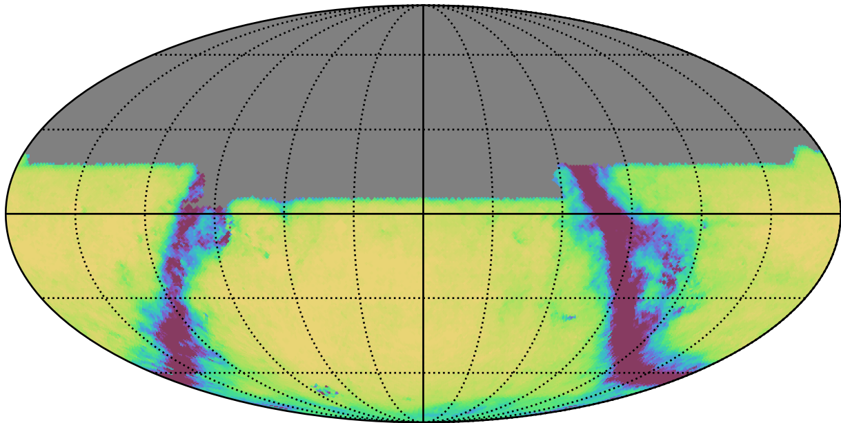
early_u_fpextra2.0_v3.4_10yrs All sky u band: Exgal_CoaddM5
