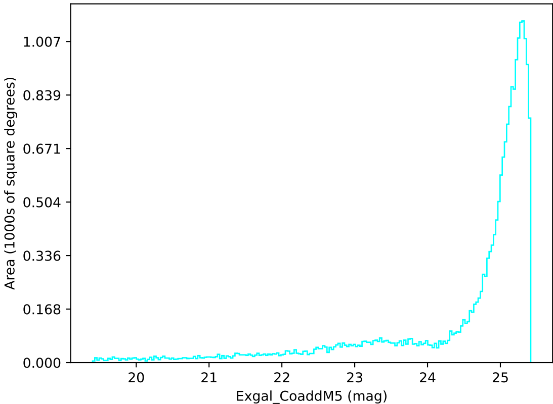
early_u_fpextra2.0_v3.4_10yrs All sky u band: Exgal_CoaddM5
