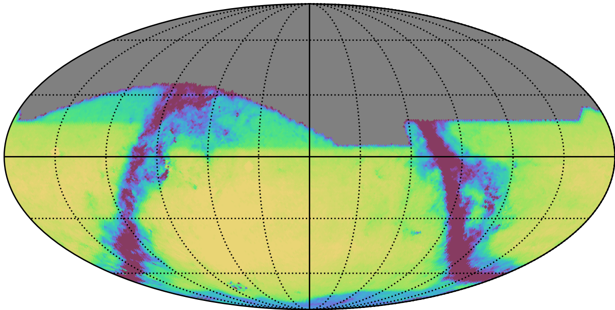
early_u_fpextra2.0_v3.4_10yrs All sky r band: Exgal_CoaddM5
