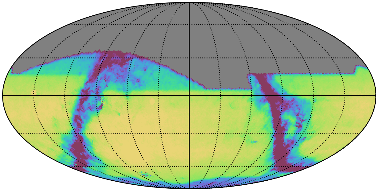
early_u_fpextra2.0_v3.4_10yrs All sky i band: Exgal_CoaddM5
