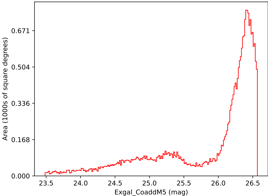
early_u_fpextra2.0_v3.4_10yrs All sky i band: Exgal_CoaddM5
