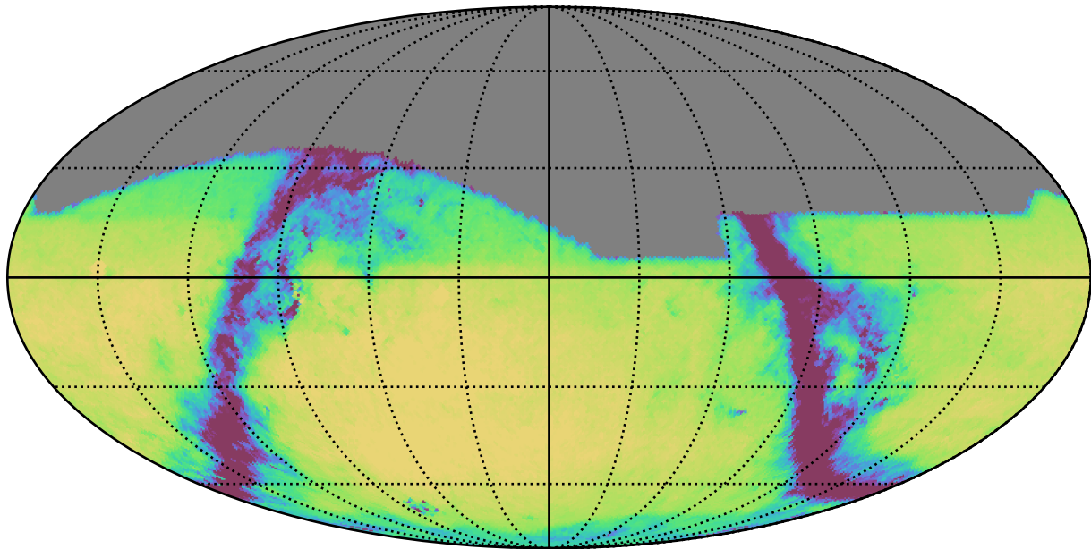
early_u_fpextra2.0_v3.4_10yrs All sky g band: Exgal_CoaddM5
