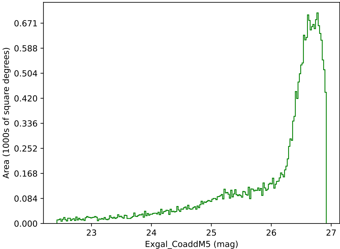
early_u_fpextra2.0_v3.4_10yrs All sky g band: Exgal_CoaddM5
