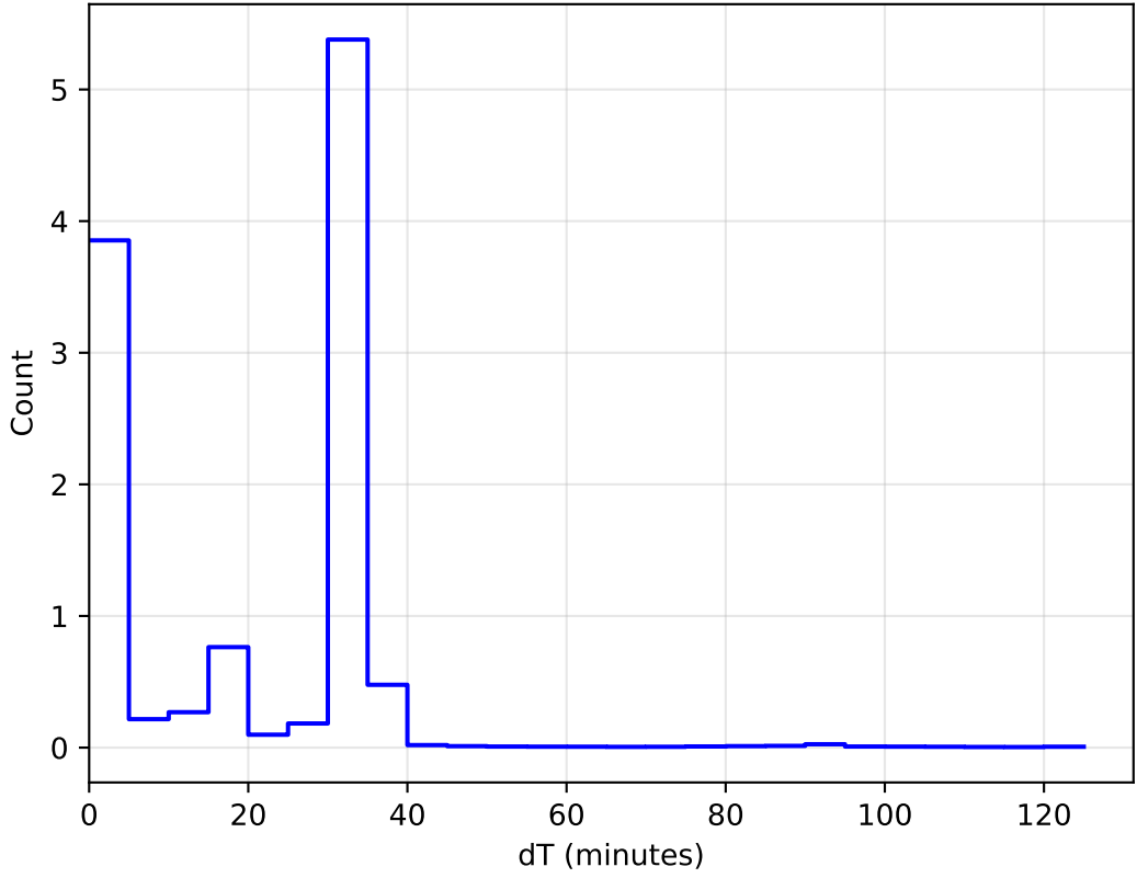
early_u_fpextra2.0_v3.4_10yrs WFD: DeltaT Histogram
