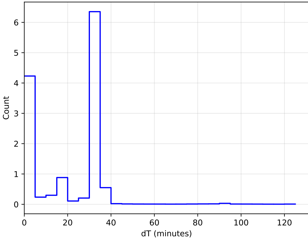
early_u_fpextra2.0_v3.4_10yrs All sky: DeltaT Histogram
