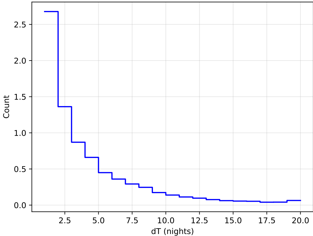
early_u_fpextra2.0_v3.4_10yrs WFD all bands: DeltaNight Histogram 1e6
