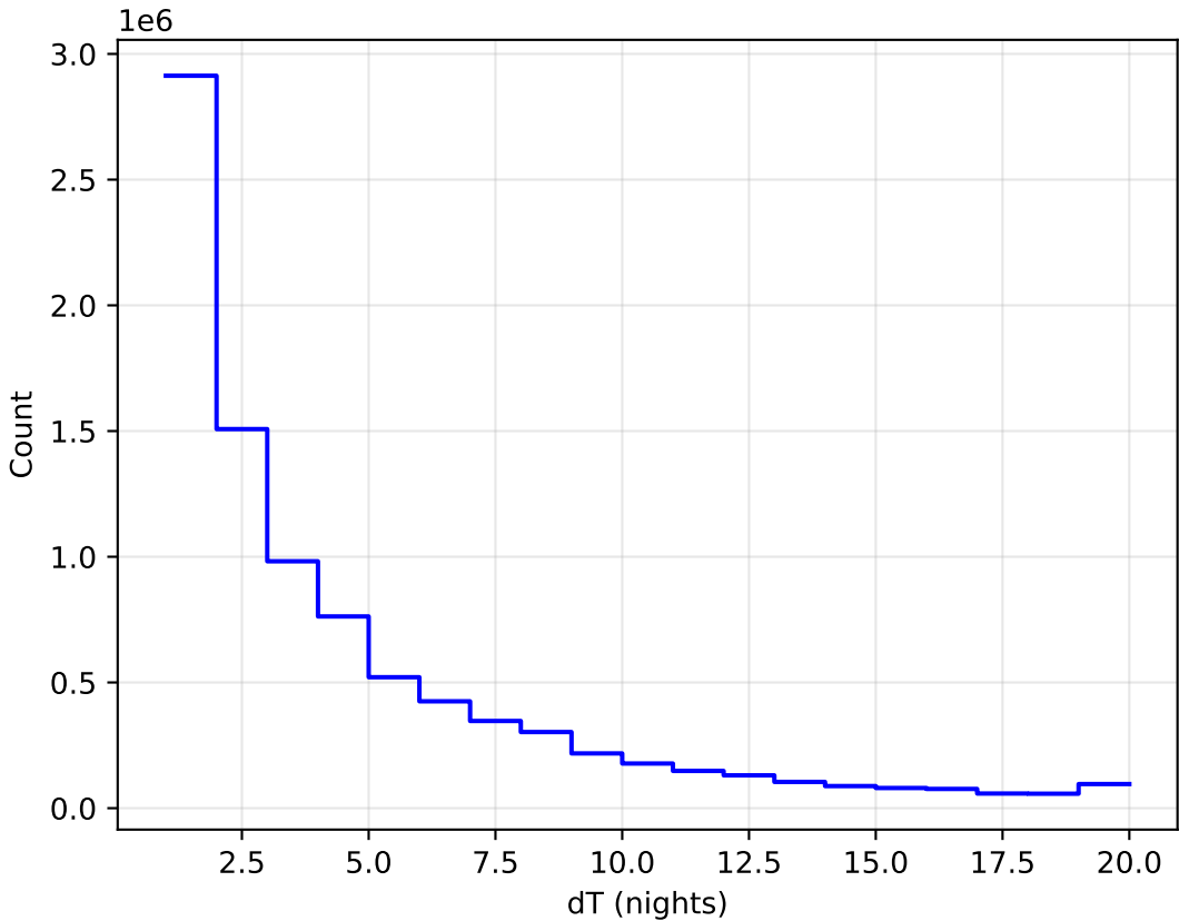
early_u_fpextra2.0_v3.4_10yrs All sky all bands: DeltaNight Histogram
