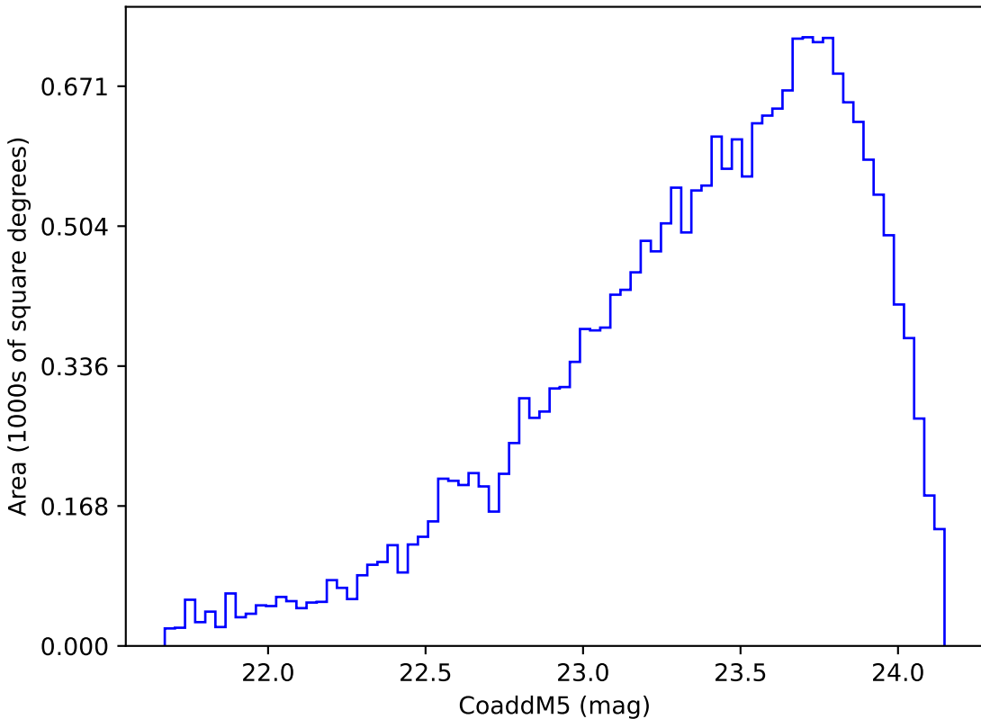
early_u_fpextra2.0_v3.4_10yrs Yr 3-4 y band: CoaddM5
