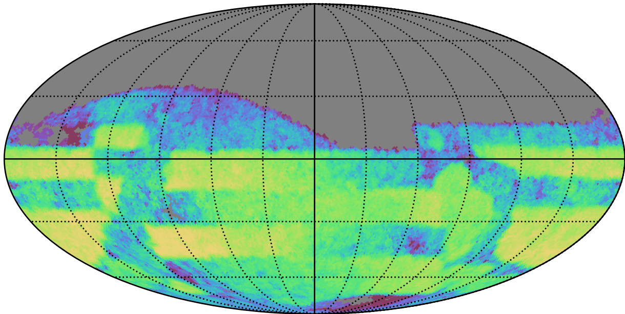
early_u_fpextra2.0_v3.4_10yrs Yr 3-4 i band: CoaddM5
