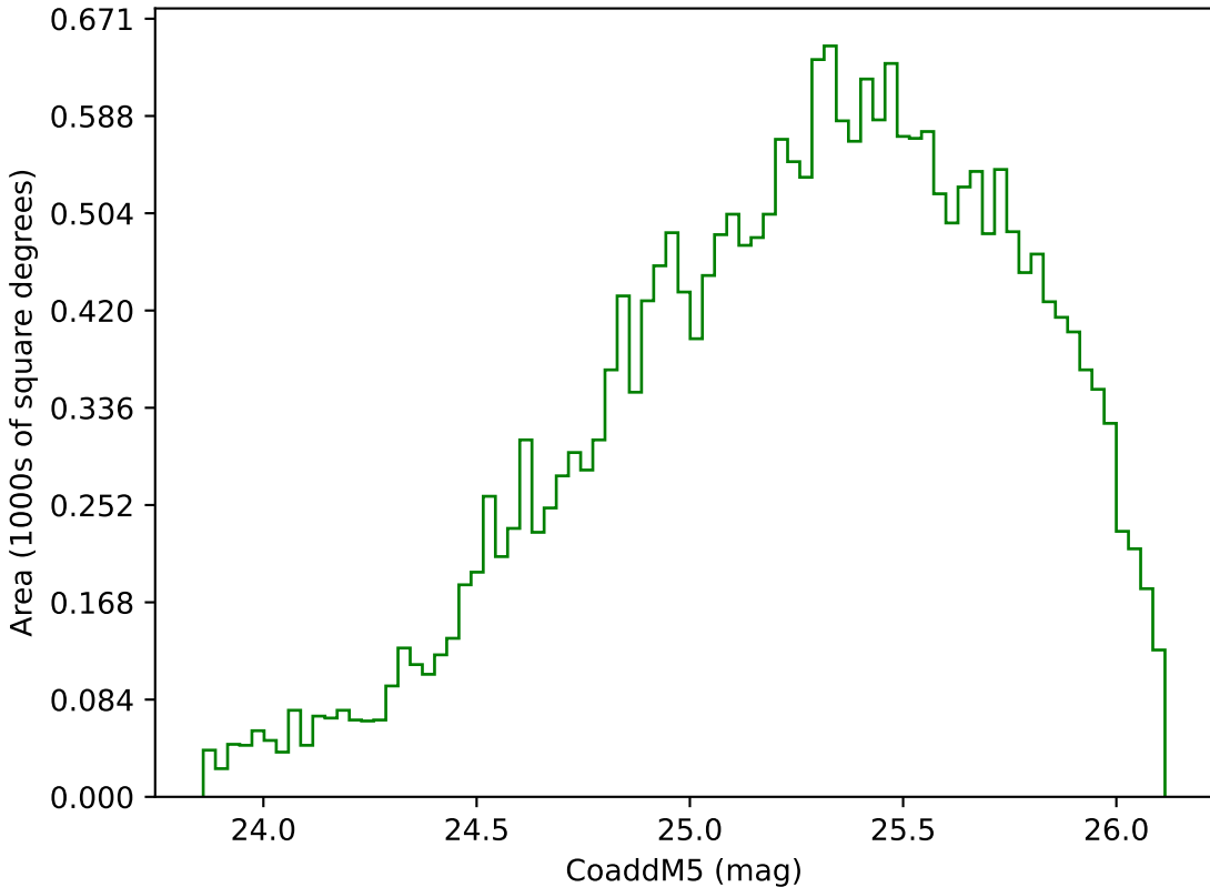
early_u_fpextra2.0_v3.4_10yrs Yr 3-4 g band: CoaddM5
