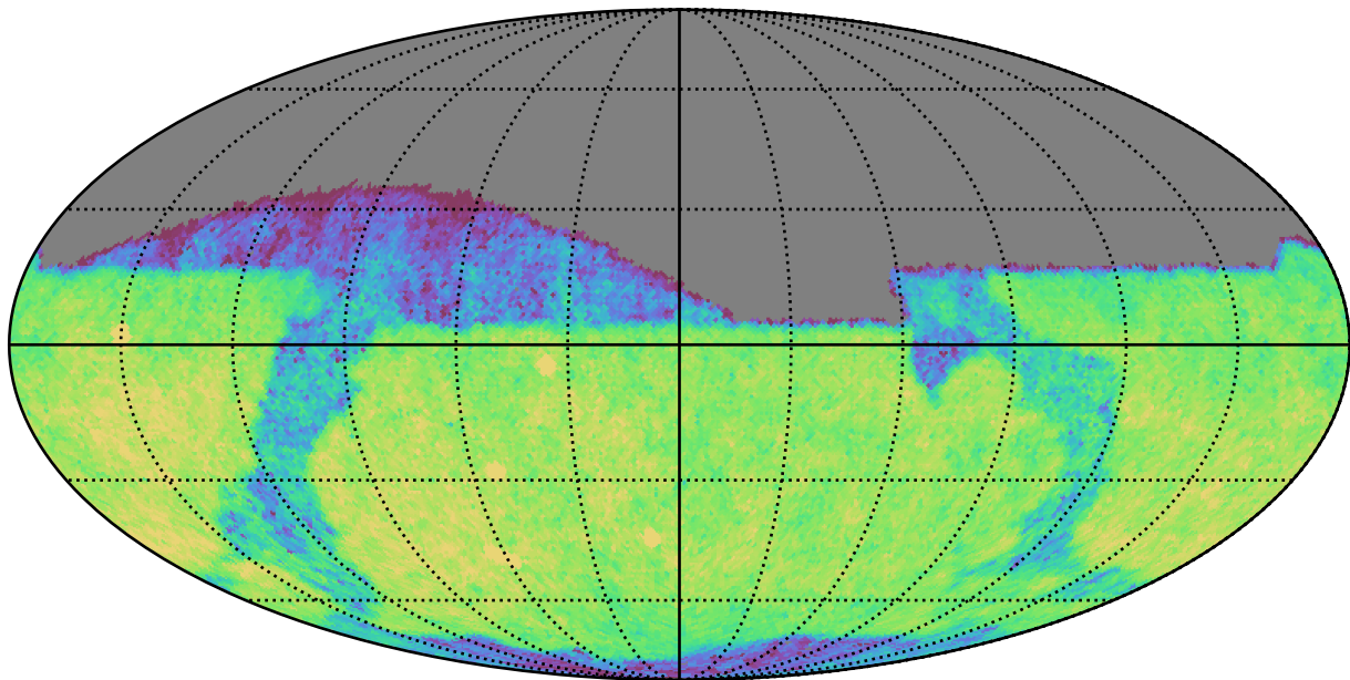
early_u_fpextra2.0_v3.4_10yrs Yr 1 z band: CoaddM5
