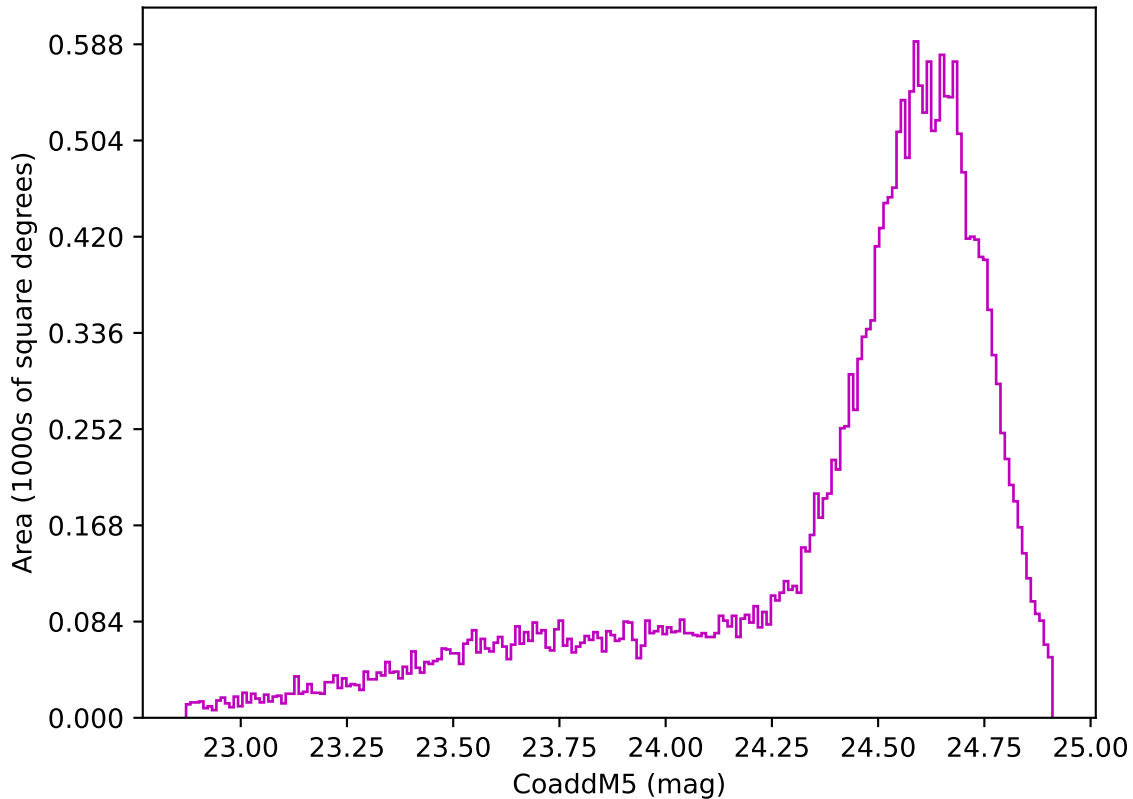
early_u_fpextra2.0_v3.4_10yrs Yr 1 z band: CoaddM5
