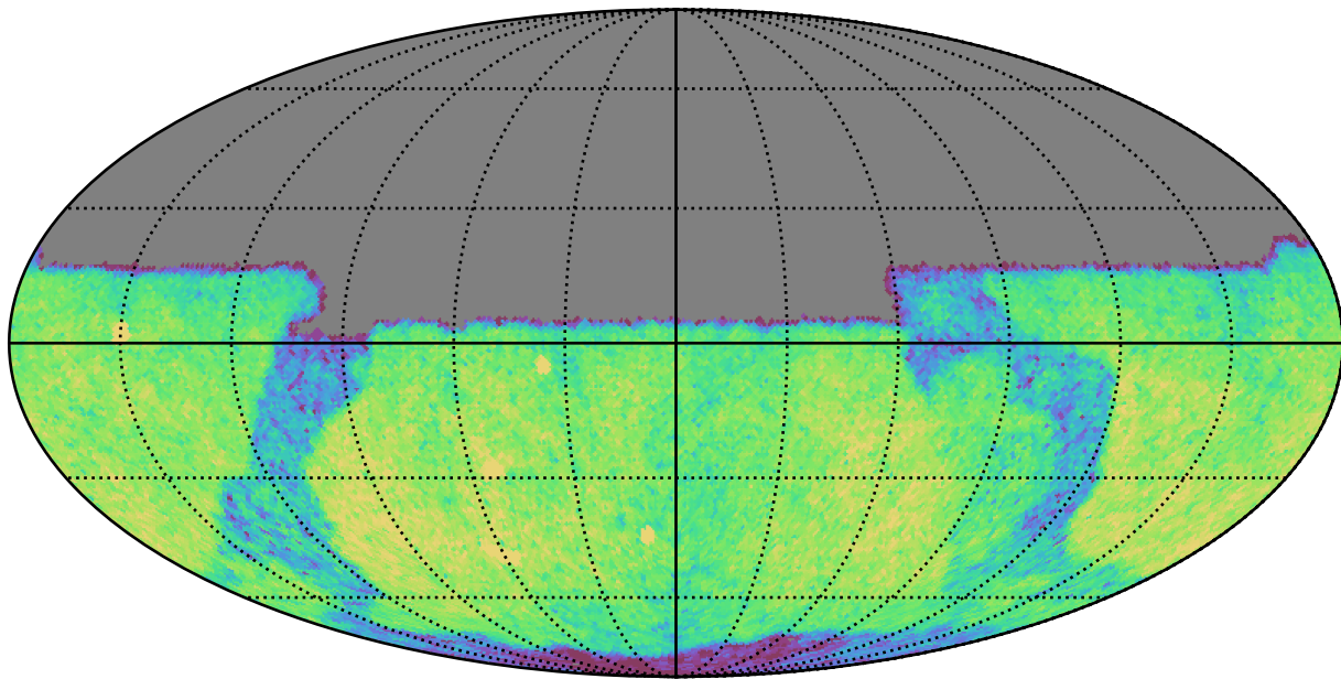
early_u_fpextra2.0_v3.4_10yrs Yr 1 y band: CoaddM5
