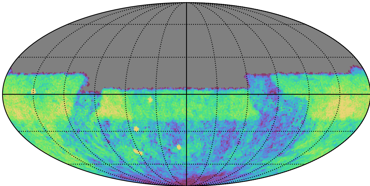
early_u_fpextra2.0_v3.4_10yrs Yr 1 u band: CoaddM5
