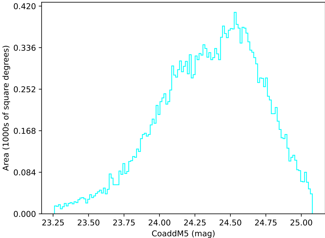
early_u_fpextra2.0_v3.4_10yrs Yr 1 u band: CoaddM5
