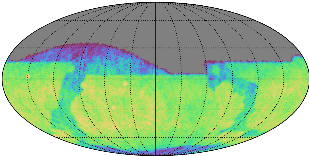
early_u_fpextra2.0_v3.4_10yrs Yr 1 r band: CoaddM5
