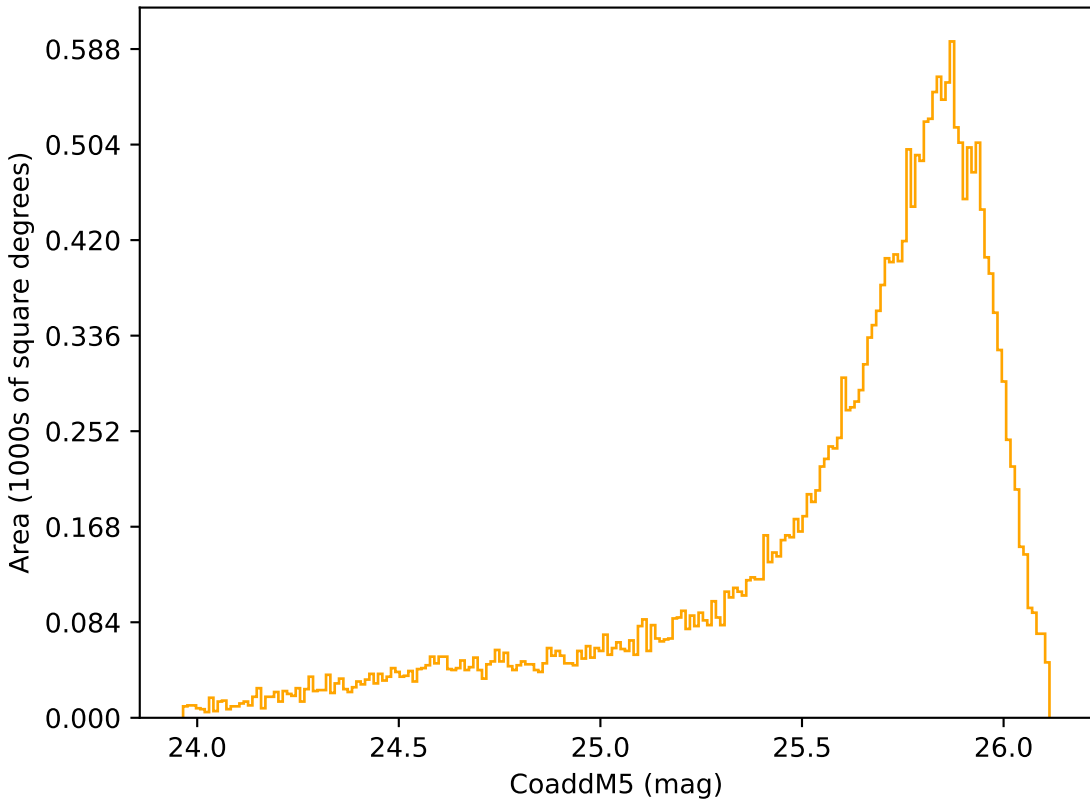
early_u_fpextra2.0_v3.4_10yrs Yr 1 r band: CoaddM5
