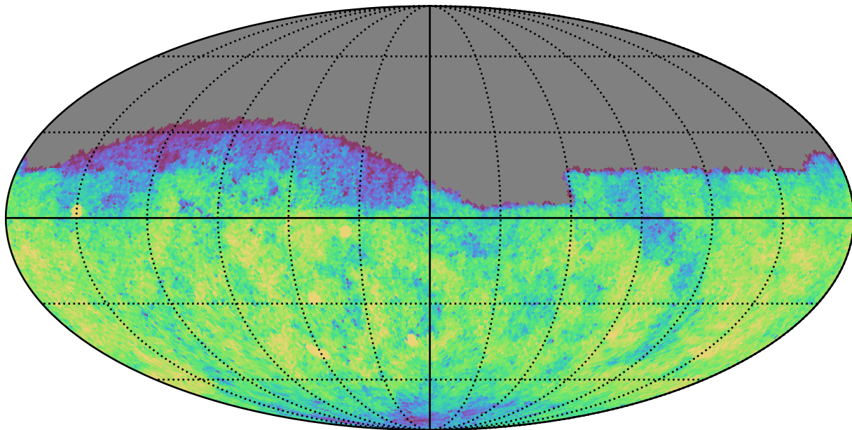
early_u_fpextra2.0_v3.4_10yrs Yr 1 g band: CoaddM5
