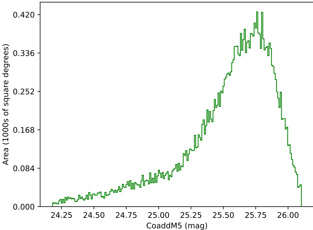
early_u_fpextra2.0_v3.4_10yrs Yr 1 g band: CoaddM5
